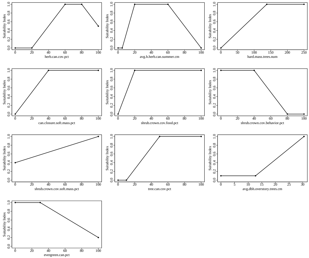
Figure 1. Suitability index graphs for variables included in the easternwildturkeyForestHardDBH35.6cm model in ecores.
